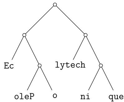
Figure 3 La corde c_2
